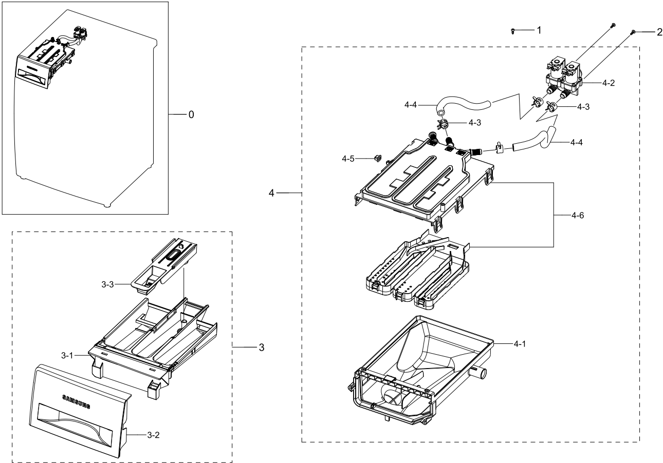
Exploded View
